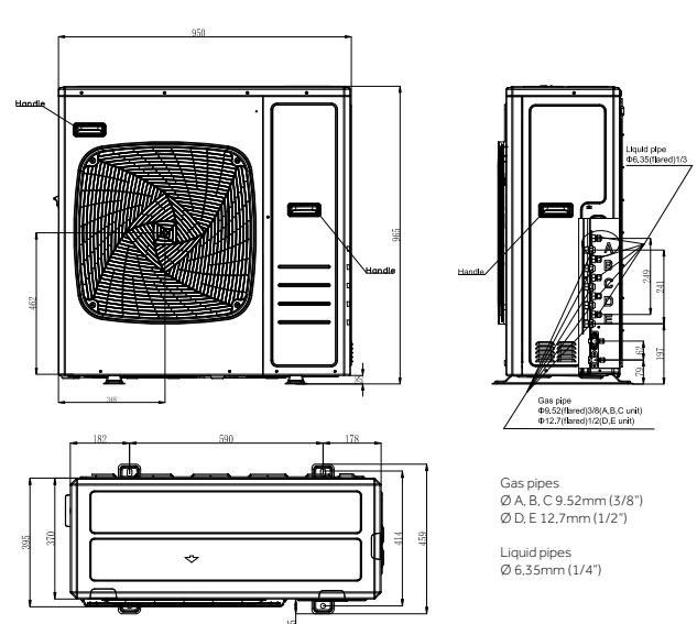
5U125S2SN1FA (5 couplings)
